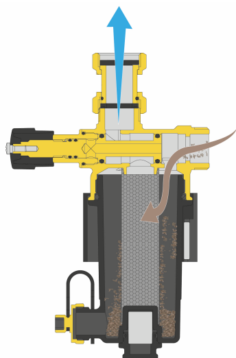
BY-PASS OPEN: Filter on
