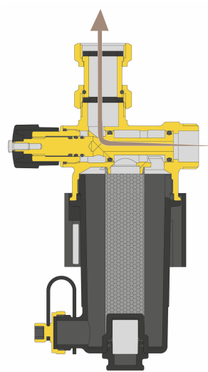
BY-PASS CLOSED: Filter off Maintenance operations are permitted.
